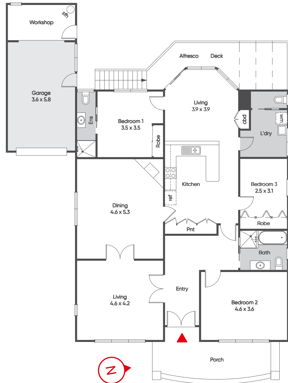
Floor plan
