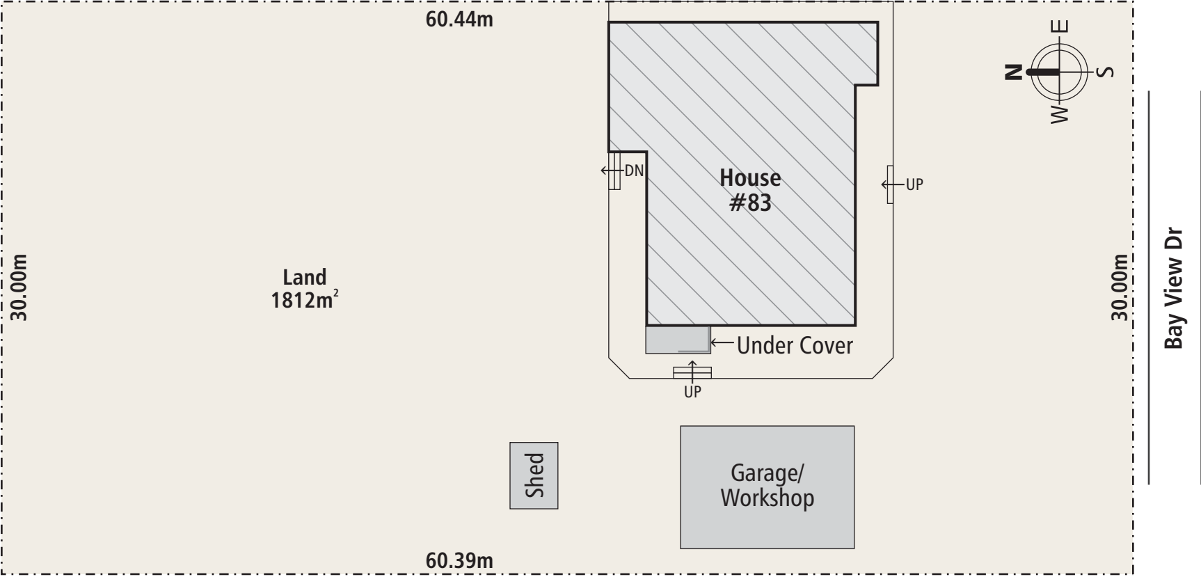
Site Plan
