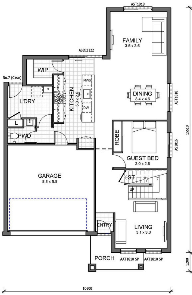
CONCERTO III-STD-GROUND FLOOR
