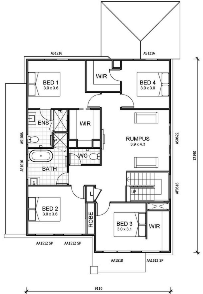
CONCERTO III-STD-FIRST FLOOR
